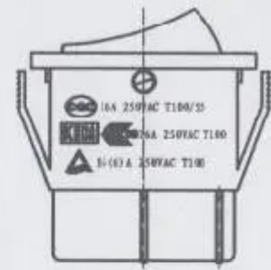
安装开孔尺寸 MOUNTING HOLE DIMENTION
